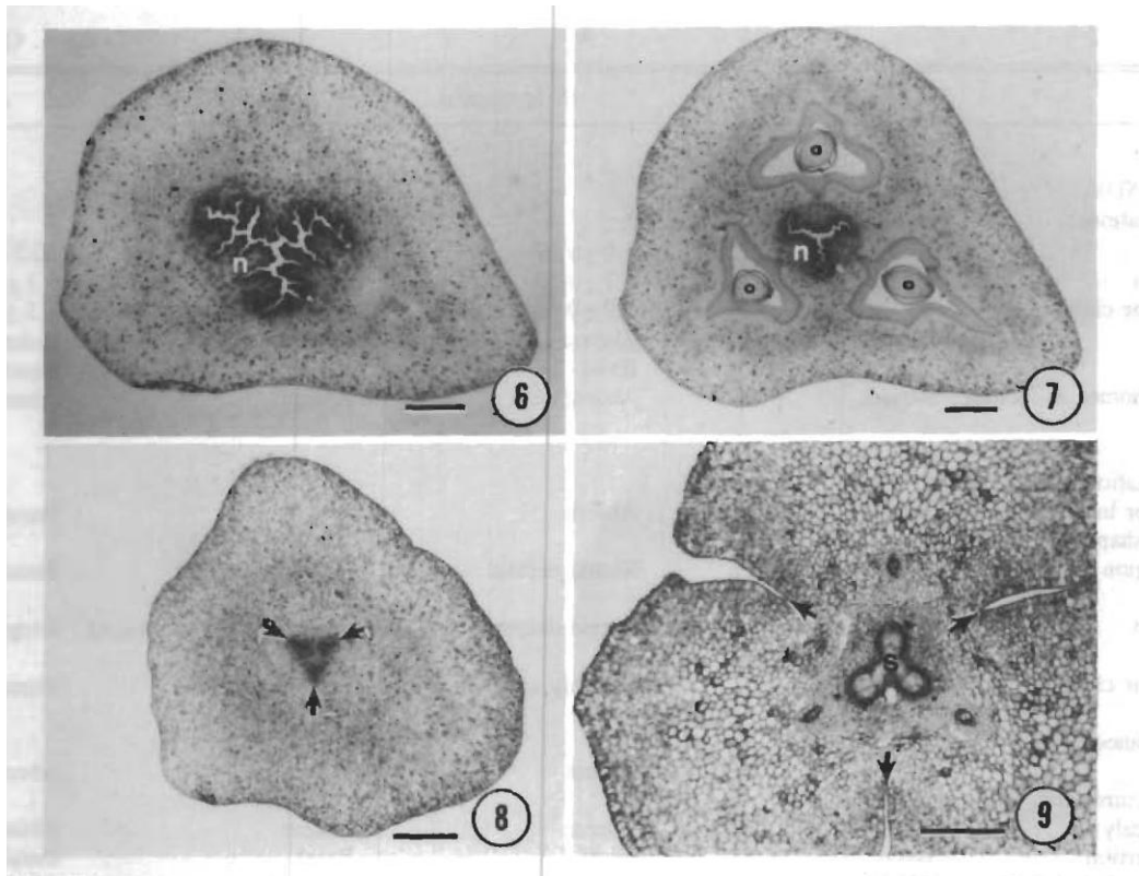
FIGS. 6-9. Heliconia indica , cross sections. Fig. 6. Sublocular region. n , nectary. Scale bar = 1.0 mm. Fig. 7. Locular region. n , nectary; o , ovule. Scale bar 1.0 mm. Fig. 8. Prolongation. Arrows point to nectary ducts. Scale
