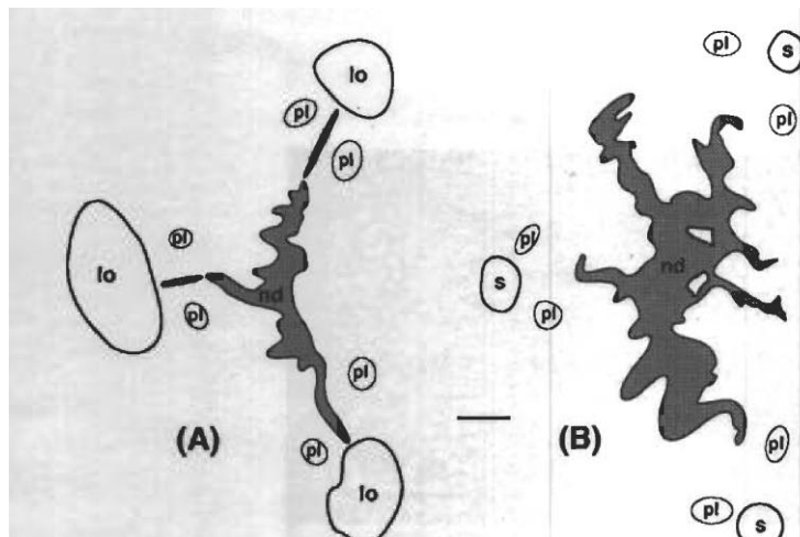
FIG. 28. Musa velutina , camera lucida drawings of nectary ducts ( nd , shaded), placental vascular bundles ( pl ), and styler canals ( s ). (A) Level of proximal prolongation. The main arms of the duct are opposite the locules. (B) Level more distal in prolongation. Arms of the nectary duct occur opposite the locules and in two of the septa. Scale bar = 0.3 mm.
