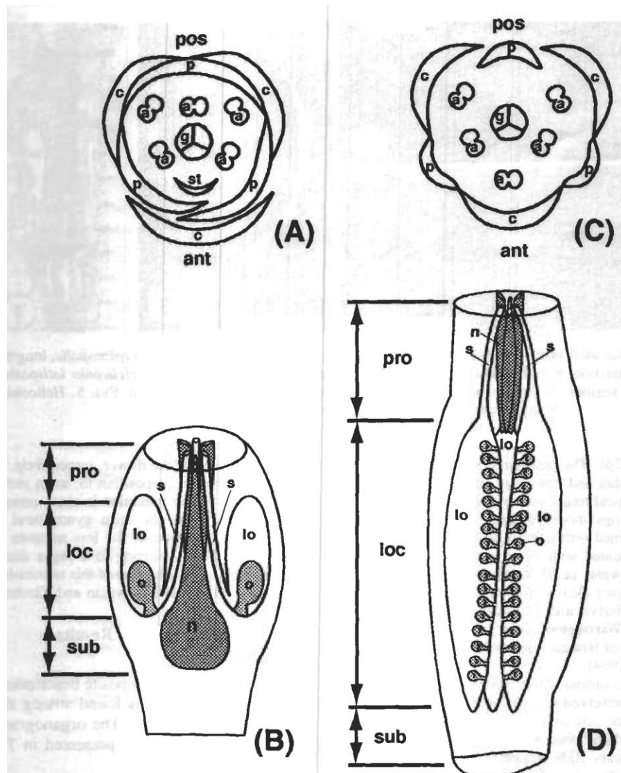
FIG. 1. Freehand diagrams of flower and ovary structure. (A) Heliconiaceae, floral diagram. (B) Heliconiaceae, ovary structure. (C) Musaceae, floral diagram. (D) Musaceae, ovary structure. a , androecial member; ant , anterior; c , sepal; g , gynoecium; lo , locule; loc , Jocular region; n , nectary; o , ovule; p , petal; pos , posterior; pro , prolongation; s , stylar canal; st , staminode; sub , sublocular region.
