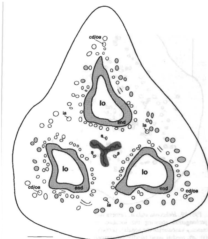
FIG. 18. Heliconia indica , camera lucida drawing, cross section of Jocular region showing the location of the vascular bundles (shaded bundles vascularize the perianth), nectary ( n ) and stylar canals ( s ). cd/oa , common carpellary dorsal/outer androecial bundle; end , endocarp; ia , inner androecial bundle; lo , locule. Scale bar = 1 mm.
