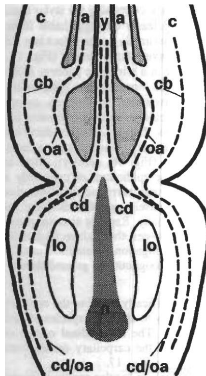
FIG. 17. Longitudinal diagram of Heliconia flower showing the path of some of the major vascular strands. a , androecial member; c , sepal; cb , median vascular strand of sepal; cd , carpellary dorsal; cd/oa , common carpellary dorsal/outer androecial strand; lo , locule; n , nectary; oa , outer androecial strand; y , style.
