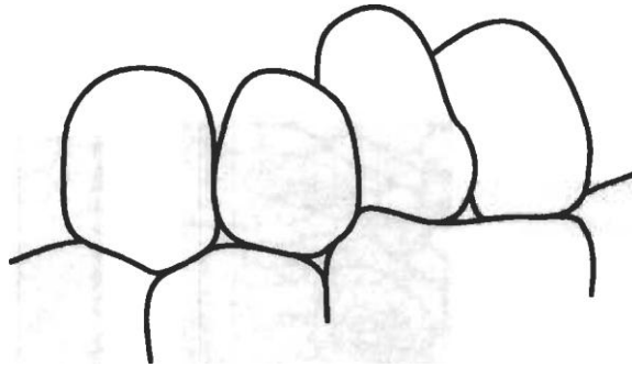
FIG. 29. Musa velutina , camera lucida drawing of a cross section of the columnar, moderately papillate epidermal cells. Scale bar = 10 \mu\text{m} .
