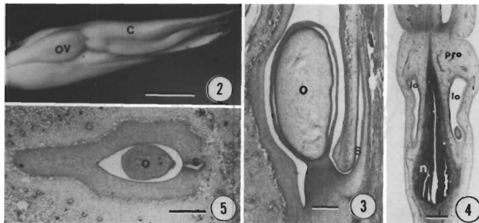
FIG. 2. Heliconia indica , mature flower. c , calyx; ov , ovary. Scale bar = 10 mm. FIG. 3. Heliconia episcopalis , longitudinal section showing insertion of ovule ( o ) and insertion of stylar canal ( s ) into locule. Scale bar = 0.25 mm. FIG. 4. Heliconia latispatha , longitudinal section of flower with three distinct regions. lo , locule; n , nectary; pro , prolongation. Scale bar = 1.0 mm. FIG. 5. Heliconia indica , cross section through base of locule with insertion of stylar canal ( s ). o , ovule. Scale bar = 0.5 mm.
